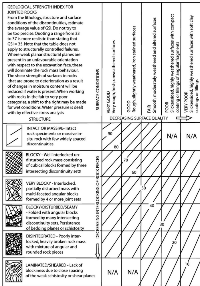
Fig. 2 A GSI chart for jointed rock mass (Marinos et al., 2005)
