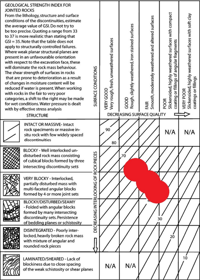
Fig. 6 A GSI chart that provided for studied stations
